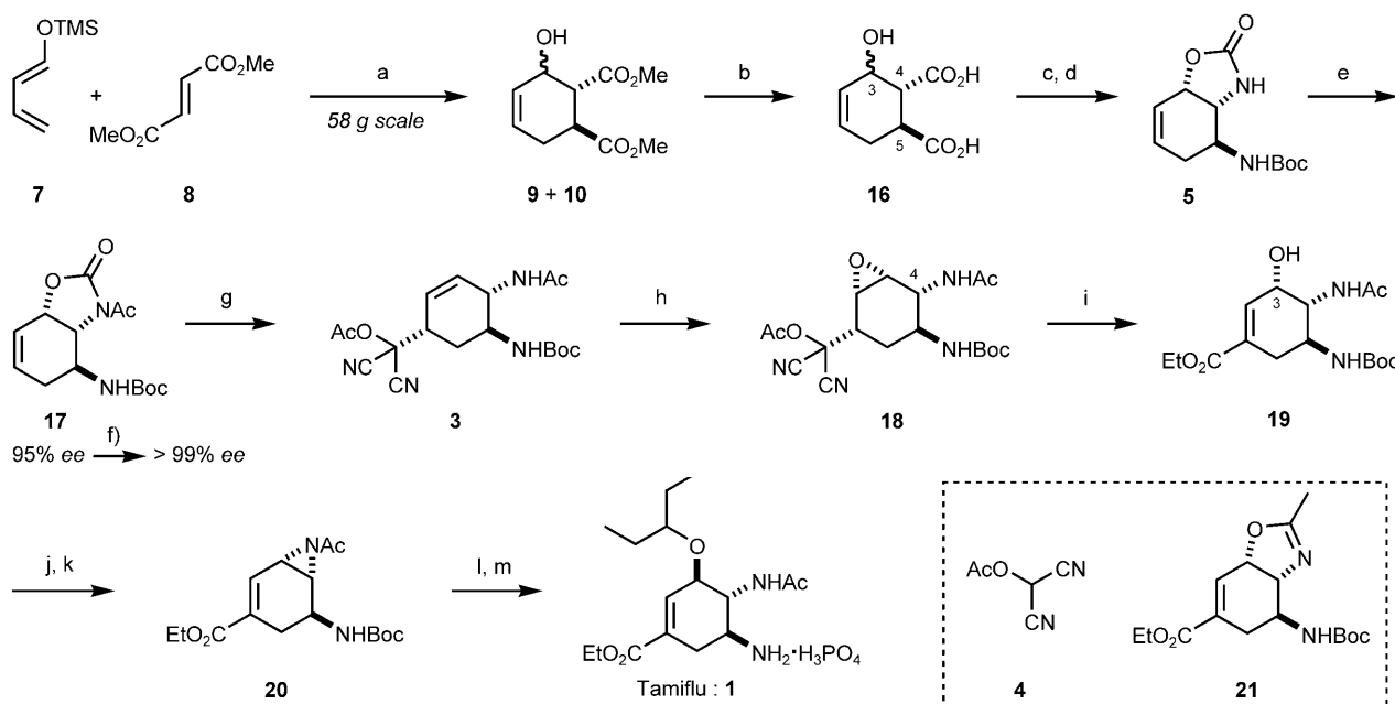
Scheme 2. Catalytic asymmetric synthesis of Tamiflu. Reagents and conditions: a) Ba(OiPr) 2 (2.5 mol %), F 2 -FujiCAPO ( 15 , 2.5 mol %), CsF (2.5 mol %), THF, −20 °C, 36–96 h; aq. 1 M HCl (91 %, 5:1, 95 % ee for 9 ); b) aq. 2 M NaOH (10 equiv), MeOH, 60 °C, 10 h; c) DPPA (3 equiv), Et 3 N (3 equiv), THF, 0 °C, 21 h (95 % (2 steps from 9 )); d) t BuOH, 80 °C, 13 h; e) Ac 2 O (2 equiv), Et 3 N (4 equiv), DMAP (10 mol %), CH 2 Cl 2 , RT, 2.5 h (ca. 98 % (2 steps)); f) Recrystallization from CH 2 Cl 2 /cyclopentyl methyl ether (1:2; 80 %); g) 4 (1.2 equiv), [Pd 2 (dba) 3 ]·CHCl 3 (2 mol %), dppf (4 mol %), toluene, 60 °C, 30 min (85 %); h) TFAA (10 equiv), urea/H 2 O 2 (20 equiv), Na 2 HPO 4 (15 equiv), CH 2 Cl 2 , 4 °C, 2 h; i) K 2 CO 3 (5 equiv), EtOH, RT, 5 h; j) DEAD (2 equiv), PPh 3 (2 equiv), p -nitrobenzoic acid (2 equiv), THF, −20 °C, 1.5 h; LiOH (3 equiv), EtOH, −20 °C, 15 min (65 % (3 steps)); k) DIAD (2.1 equiv), Me 2 PPh (2.1 equiv), Et 3 N (21 mol %), CH 2 Cl 2 , 4 °C, 10 min (76 %); l) BF 3 ·OEt 2 (1.5 equiv), 3-pentanol, −20 °C, 15 min (75 %); m) TFA; H 3 PO 4 (73 %). DPPA = diphenylphosphoryl azide; DMAP = 4-dimethylaminopyridine; dba = dibenzylideneacetone; dppf = bis(diphenylphosphanyl)ferrocene; TFAA = trifluoroacetic anhydride; DEAD = diethyl azodicarboxylate; DIAD = diisopropylazodicarboxylate; TFA = trifluoroacetic acid; Boc = tert -butoxycarbonyl; Ac = acetyl.
